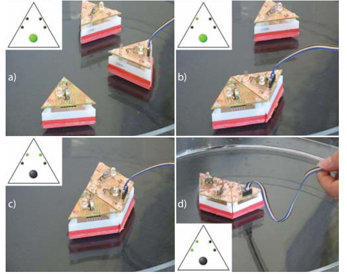
Fig. 8. Example for Tribolon state transition. The inset indicates the state as seen by the active module during the experiment, and its action (small circles: dark (no neighbor) and bright (connected neighbor); large circle: dark (motor stopped) and bright (motor running)): a) no neighbor: motor running, b) L: motor running, c) RL: motor stopped, d) LL: motor stopped. (see Fig. 6)
