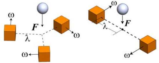
Fig. 4. Nominal attractive configurations of three field sources (without loss of generality) on a facet, and two field sources on an edge. Each field source is at a distance of \lambda (units m) from the nominal attraction axis. Although each field source is depicted with an \omega vector, in practice we duty cycle them so that only one field source is active at any given instant.
