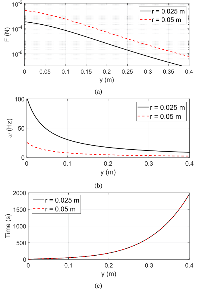
Fig. 9. (a) The maximum achievable attractive force F induced by two m = 40 \text{ A} \cdot \text{m}^2 rotating dipole fields with \lambda = 0.2 \text{ m} on copper spheres of different radii at each location y along the nominal attraction axis, (b) the frequency \omega that creates the maximum achievable attractive force, (c) and the time it takes for the sphere to be pulled to y = 0 , starting at rest at each y .
