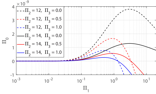
Fig. 7. Magnitude of nondimensional attractive force ( \Pi_0 ) as a function of \Pi_1 for different combinations of \Pi_2 and \Pi_3 . A negative \Pi_0 indicates repulsion. Note: \Pi_3 = 0 corresponds to \phi = 0^\circ and \Pi_3 = 1 corresponds to \phi = 45^\circ .
