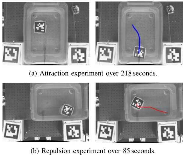
Fig. 12. Example attraction and repulsion experiments, with initial (left) and final (right) conditions shown. The experimental setup comprises two Omnimagnets placed 0.4 m apart and a pool of water with a raft, equipped with a fiducial marker, carrying a 20-mm-radius copper sphere. See Supplemental Video 3. Note: the fiducial markers on the two Omnimagnets are not being utilized here. (a) Attraction experiment over 218 seconds. (b) Repulsion experiment over 85 seconds.
