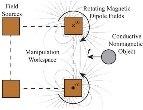
Fig. 1. Schematic depicting a conductive nonmagnetic object outside of the convex hull of a manipulation workspace being pulled into the workspace by a force f induced by multiple magnetic dipole fields rotating with frequency \omega .
