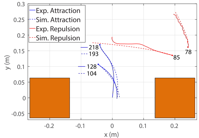
Fig. 13. Experimental and simulated trajectories. Initial positions are shown as dots. The Omnimagnets are depicted as copper squares. For the attraction experiments, the time (in seconds) to reach y = 0 is indicated. For the repulsion experiments, the simulation was run for the same amount of time as the respective experiment, which is indicated.
